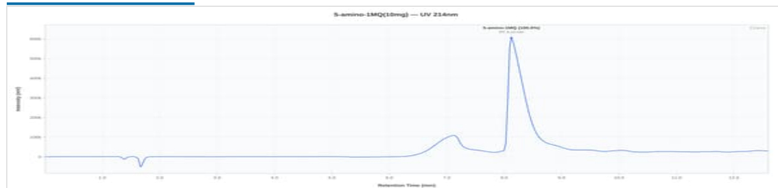
5 Amino 1mq 10mg - 5AMI-01: UV Chromatogram
